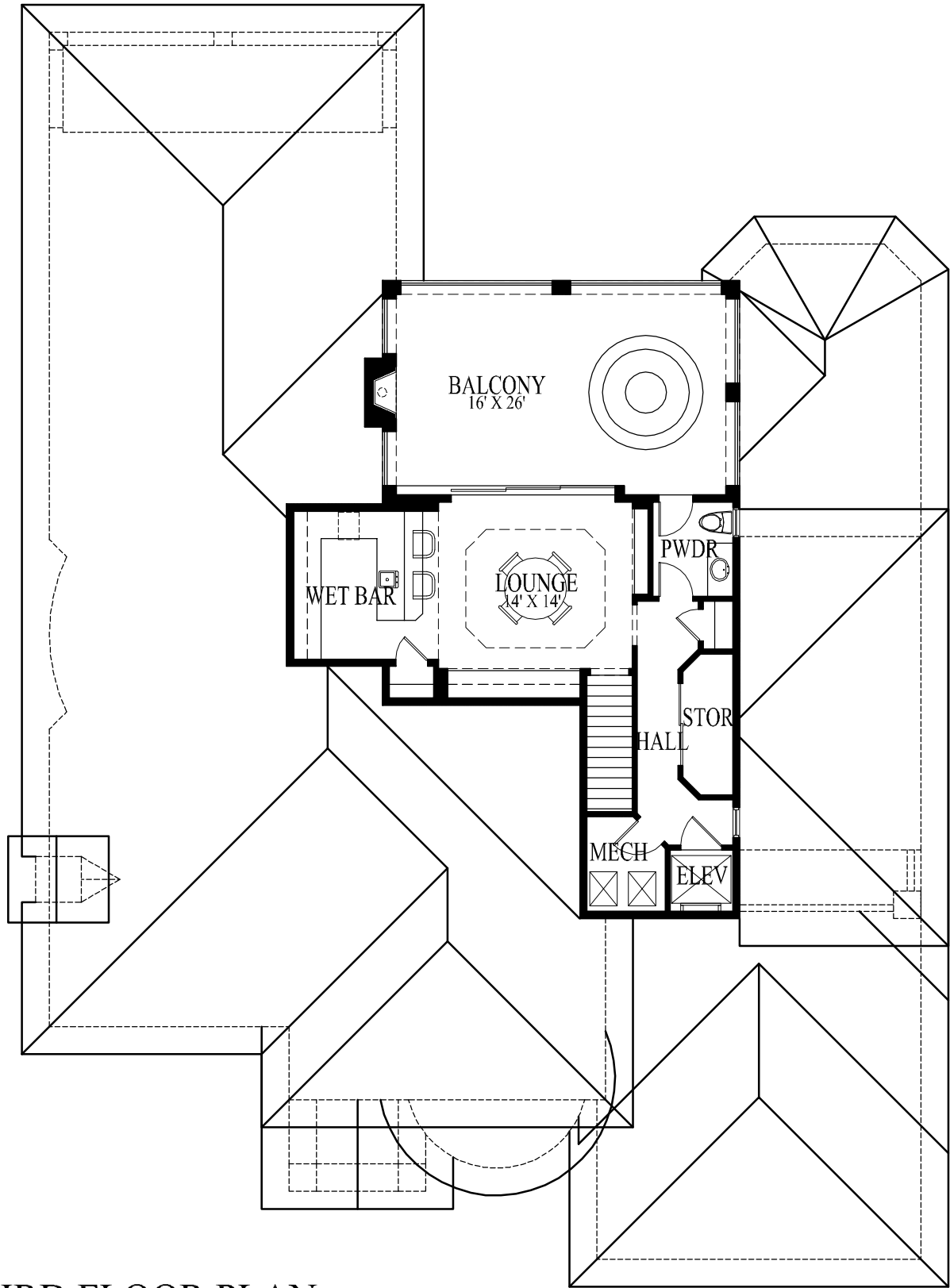
THIRD FLOOR PLAN 643 SF A/C
