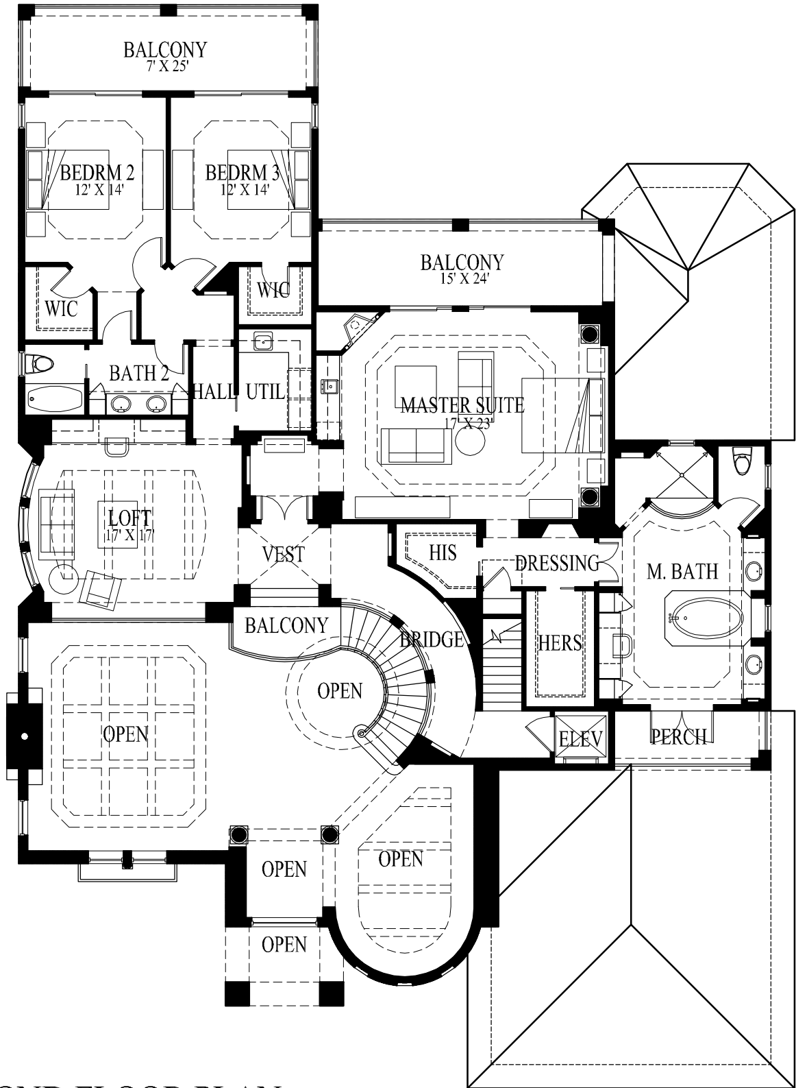
SECOND FLOOR PLAN 2011 SF A/C
