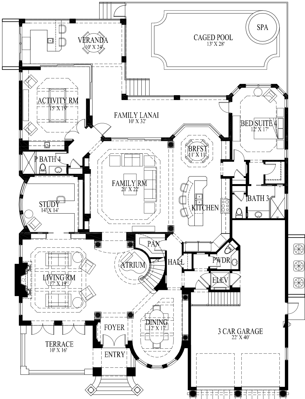
GROUND FLOOR PLAN 3120 SF A/C
